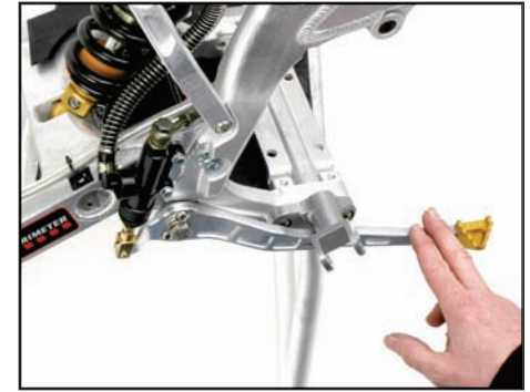
16. Push on brake pedal and check for proper operation.
