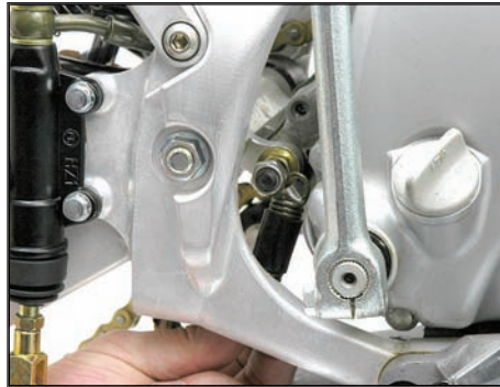
12. Install the brake pedal spring on the top bolt mount.
